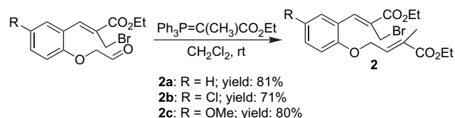
Scheme 3. Synthesis of substrates 2a–c .
