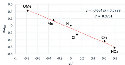
Figure 4. Hammett plot for substituted arenesulfonyl azides.
