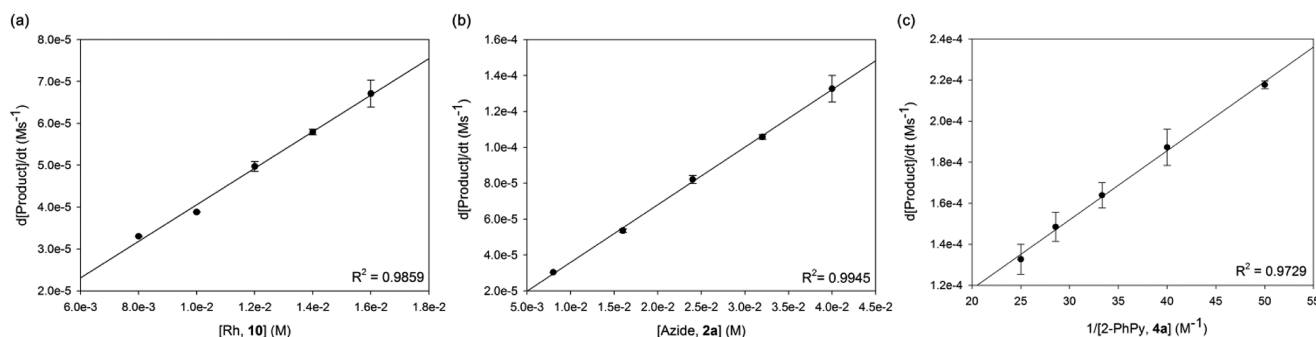
Figure 3. (a) Plot of initial rate versus [10] showing the first order. (b) Plot of initial rate versus [2a] ( p -toluenesulfonyl azide) showing the first order. (c) Plot of initial rate versus 1/[4a] (2-phenylpyridine) showing the inverse first order.
