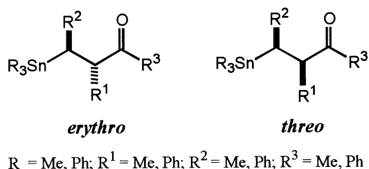
Fig. 1. Stereochemistry of compounds 6–16 .
