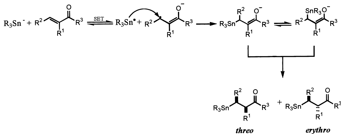
Scheme 1. Reaction of triphenyl- and trimethylstannyl-potassium with enones 1–5.
