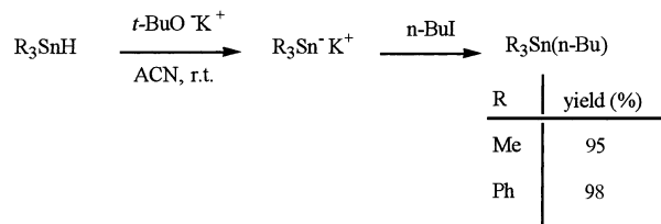
Fig. 2. Results obtained in the generation of triphenyl- and trimethylstannylpotassium.
