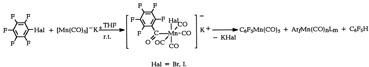
Scheme 4. Rearrangement of haloacylmanganates.
