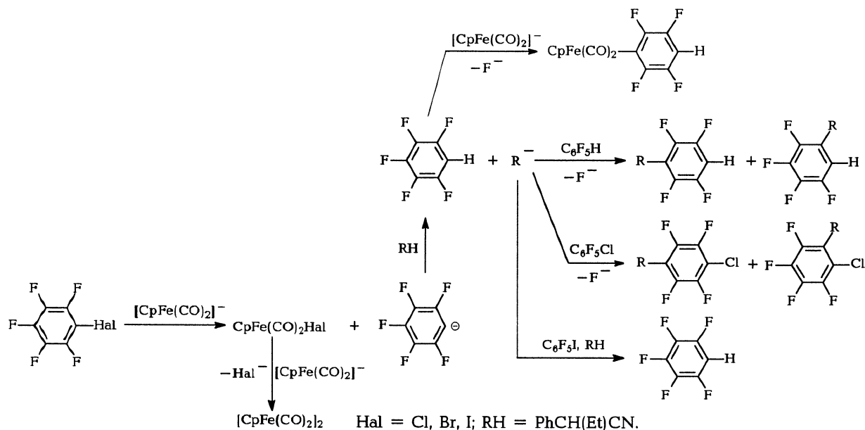
Scheme 3. Trapping of [\text{C}_6\text{F}_5]^- carbanion by CH-acid.
