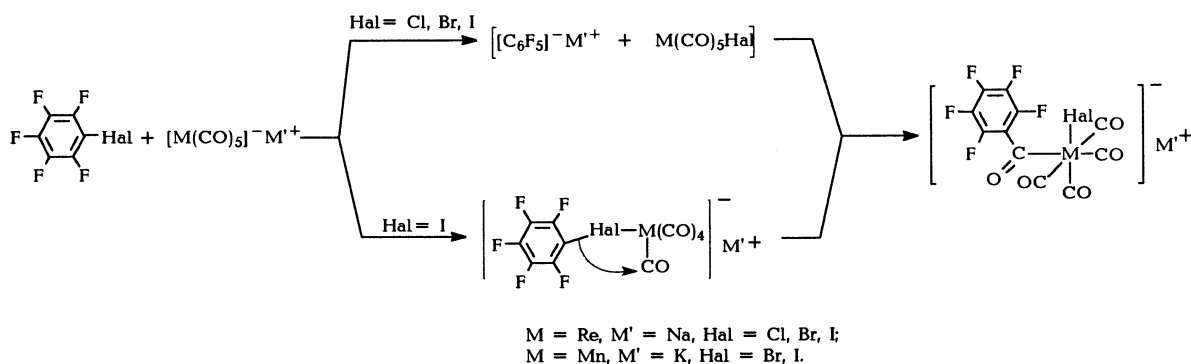
Scheme 6. Alternative mechanisms of haloacylmetallate formation.
