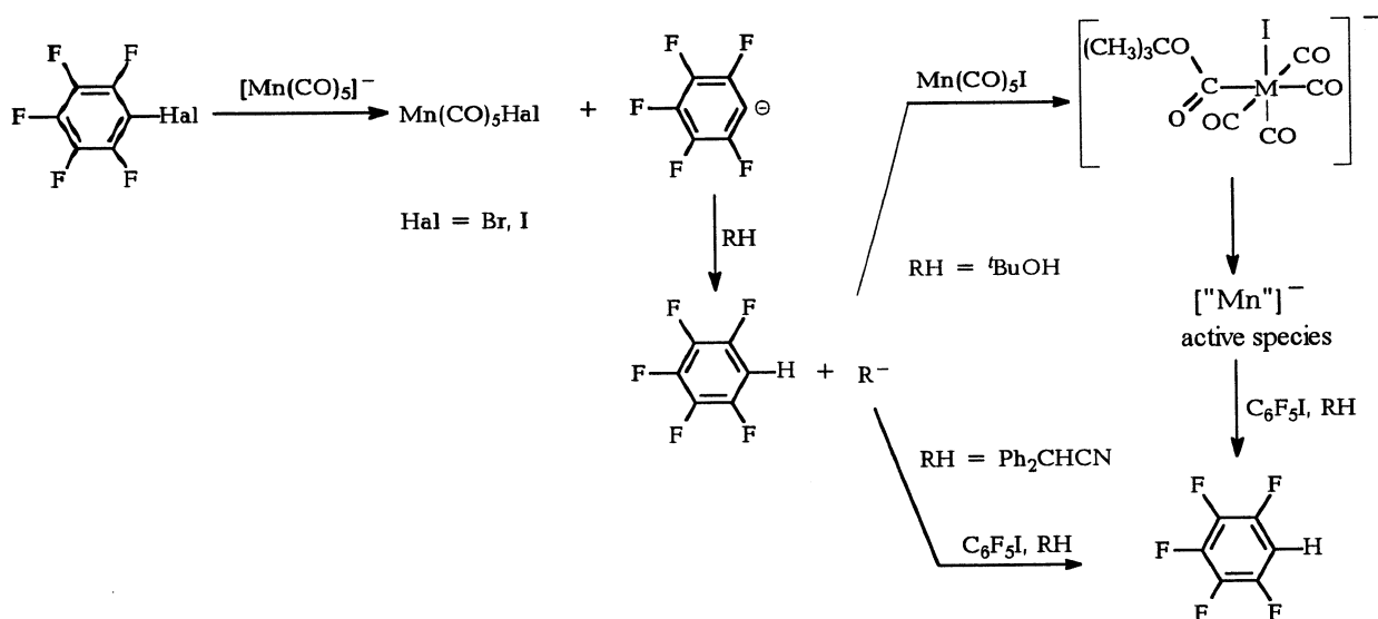
Scheme 5. Trapping of [C_6F_5]^- anion in the reaction of [Mn(CO)_5]K with C_6F_5Hal .
