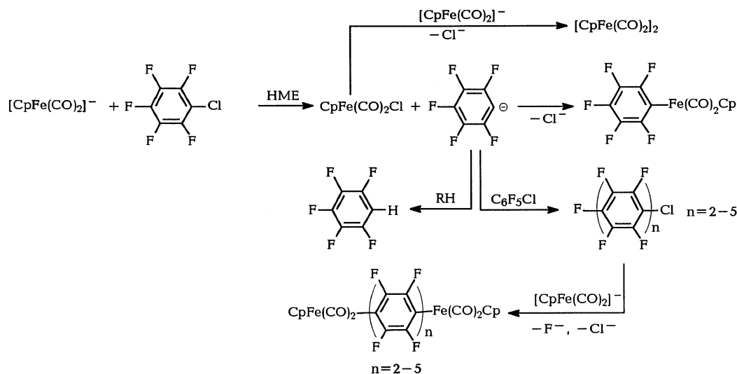
Scheme 1. Halophilic mechanism for the reaction of C_6F_5Cl with [CpFe(CO)_2]^- anion.
