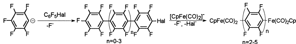
Scheme 2. Reaction sequence producing perfluoropolyphenyls.
