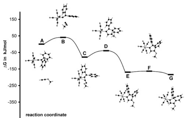
Figure 3. Gibbs free energy profile for the reaction of [(\text{CO})_5\text{Cr}=\text{C}=\text{CHPh}] with \text{HC}\equiv\text{CMe} at 298 K (see also Scheme 9).
