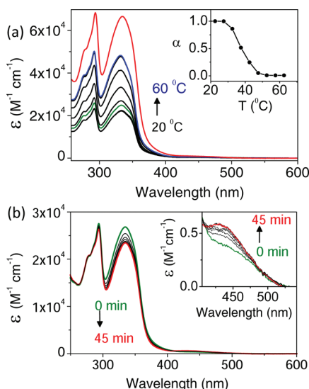
Figure 1. (a) UV/vis absorption spectral changes of 4 ( 1 \times 10^{-5} M) in chloroform (red), in cyclohexane at 20 °C (black), and in cyclohexane at 60 °C (blue). Inset shows the plot of fraction of aggregates ( \alpha ) versus temperature (in cyclohexane, \lambda = 330 nm). (b) Spectral changes of 4 upon photoirradiation in cyclohexane ( 1 \times 10^{-5} M) using 350 nm light at 25 °C. The inset zooms in on the region between 400 and 525 nm.
