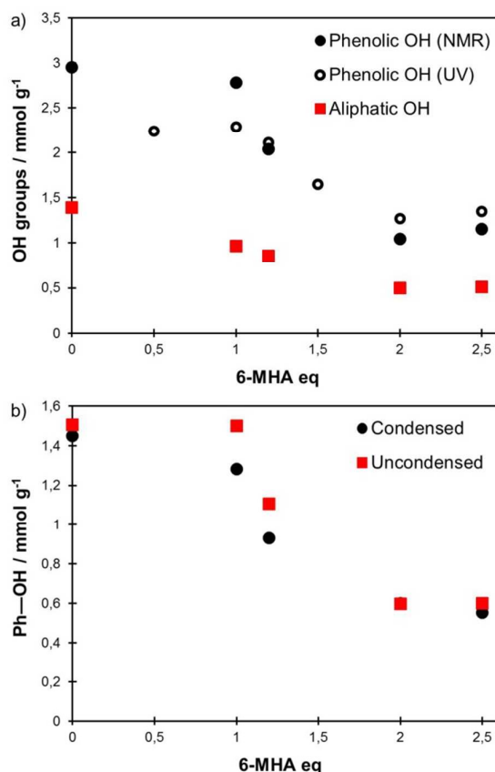
Figure 5. Content in phenolic and aliphatic OH groups of the lignins functionalized with increasing amount of 6-MHA (a) and evolution of the content in condensed and uncondensed phenolic OH groups (b).
