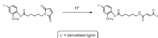
Scheme 3. Possible opening of the maleimide ring under the acidic conditions of the phosphorylation reaction, causing the observed increase in carboxyl groups by ^{31}\text{P} NMR.
