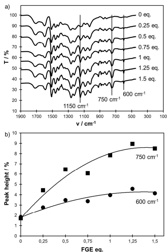
Figure 4. FTIR spectra of the functionalized lignins, depending on the amount of FGE used for functionalization (a) and evolution of the furan peaks heights with the amount of FGE used for functionalization (b).
