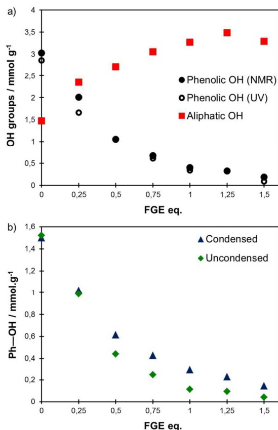
Figure 1. Content in phenolic and aliphatic OH groups of the lignins functionalized with increasing amount of FGE (a) and evolution of the content in condensed and uncondensed phenolic OH groups (b).
