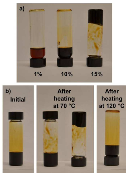
Figure 9. Solutions of functionalized lignins (furan/maleimide 1:1 w/w) in DMSO (1, 10 or 15% w/w) after heating at 70 °C (a) and 15% w/w solution before and after heating at 70 °C, and after heating at 120 °C (b)
