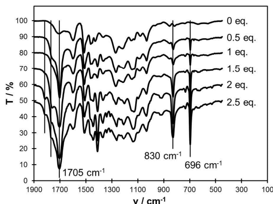
Figure 8. FTIR spectra of the functionalized lignins, depending on the amount of 6-MHA used for functionalization
