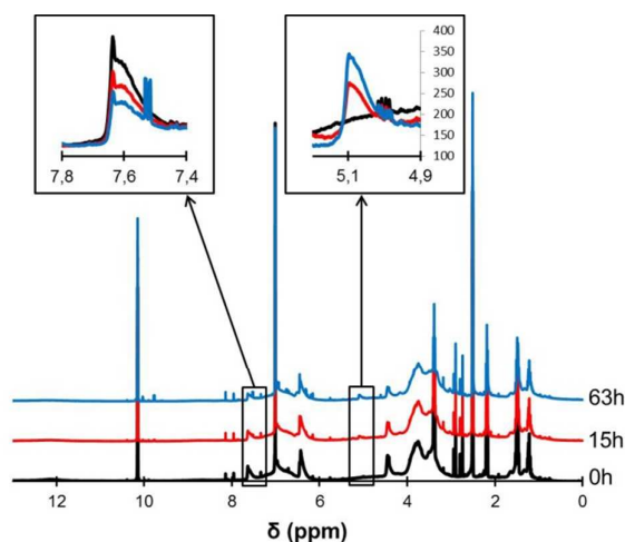
Figure 10. 1 H NMR spectra of F50_M50, measured after different time at 70 °C.
