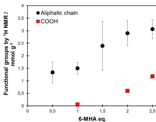
Figure 7. Functional groups calculated from 1 H NMR. Spectra are available as supplementary information (Figure S6). The aliphatic chain has been calculated as the average of the integration regions 2.10 – 2.30 ppm (2H) and 1.00 – 1.80 ppm (6H).
