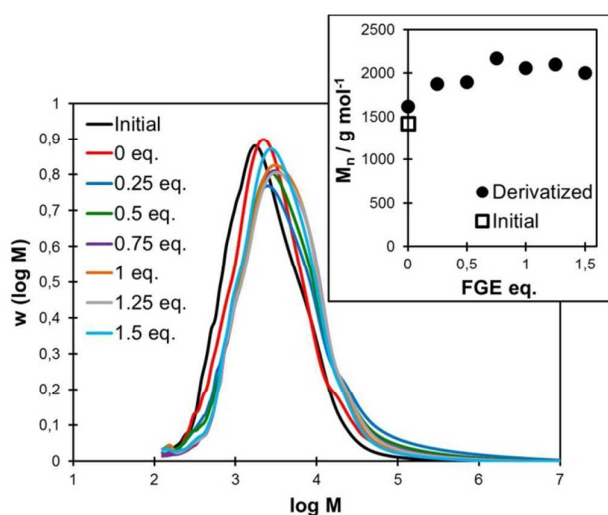
Figure 3. Molecular weight distributions of the lignins functionalized with 0 to 1.5 eq. FGE. The inset shows the evolution of M_n with the amount of FGE used for functionalization.
