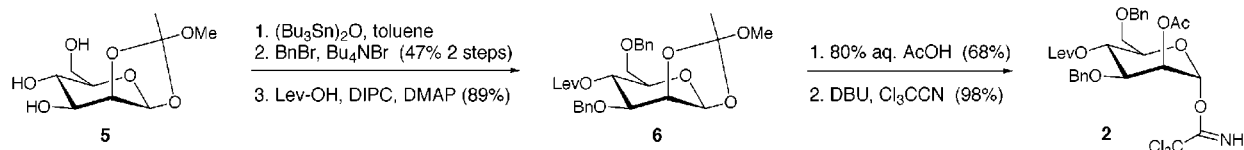
Scheme 1. Synthesis of Mannosyl Trichloroacetimidate 2
