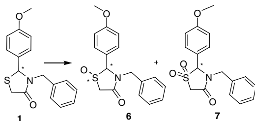
Fig. 3. sulfide oxidation of 1 .
