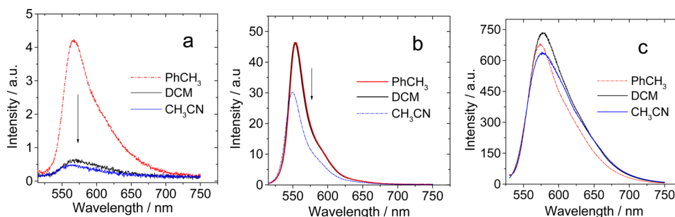
Figure 4. Fluorescence emission spectra: (a) B-1 ( \lambda_{\text{ex}} 508 nm); (b) L-3 ( \lambda_{\text{ex}} 508 nm); (c) L-1 ( \lambda_{\text{ex}} 515 nm). Optically matched solutions were used. Conditions: 20 °C.
