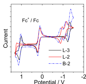
Figure 6. Cyclic voltammograms of L-3, L-2, and B-2. Ferrocene (Fc) was used as internal reference ( E_{1/2} = +0.64 V (Fc + /Fc) vs standard hydrogen electrode). Conditions: in deaerated CH 2 Cl 2 solutions containing 0.5 mM photosensitizers with the ferrocene, 0.10 M Bu 4 NPF 6 as supporting electrolyte, Ag/AgNO 3 reference electrode, scan rate 50 mV/s, 20 °C.
