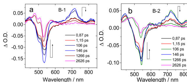
Figure 11. Ultrafast transient absorption spectra of (a) B-1 and (b) B-2. Conditions: c = 1.0 \times 10^{-5} M in toluene, excited with 530 nm femtosecond pulsed laser, 20 °C.
