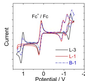
Figure 5. Cyclic voltammograms of L-3, B-1, and L-1. Ferrocene (Fc) was used as internal reference ( E_{1/2} = +0.64 \text{ V} ( \text{Fc}^+/\text{Fc} ) vs standard hydrogen electrode). Conditions: in deaerated \text{CH}_2\text{Cl}_2 solutions containing 0.5 mM photosensitizers with the ferrocene, 0.10 M \text{Bu}_4\text{NPF}_6 as supporting electrolyte, \text{Ag}/\text{AgNO}_3 reference electrode, scan rate 50 mV/s, 20 °C.
