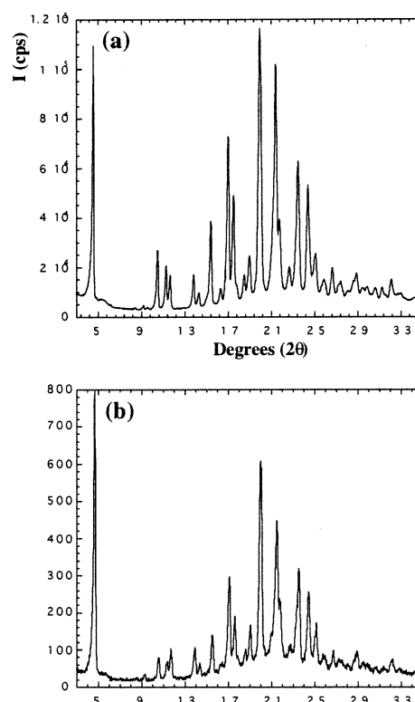
Figure 10. X-ray diffraction patterns of powder samples of 1c ; (a) 0% ee and (b) 99% ee.
