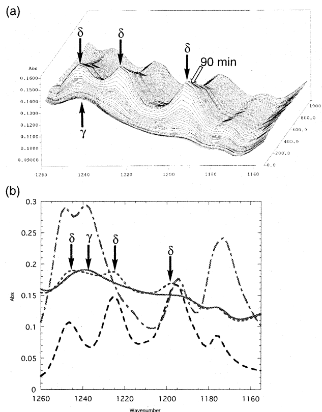
Figure 5. (a) Time development of the in situ FTIR spectra monitored by means of React IR spectroscopy during crystallization from the supersaturated EtOH solution of (±)- 1a (0.1 mol/L). (b) Comparison of spectra at the beginning (solid line, —) and the end (dotted line, ...) of crystallization, taken from the above spectra, with the spectra in the solid state of (±)- 1a (dashed line, ---, \delta -form crystal structure) and (±)- 3 (dashed and dotted line, -.-.-, \gamma -form crystal structure). Black arrows indicate the absorptions corresponding to the \delta - or \gamma -form supramolecular structure. A white arrow points the absorption at 90 min after crystallization began.
