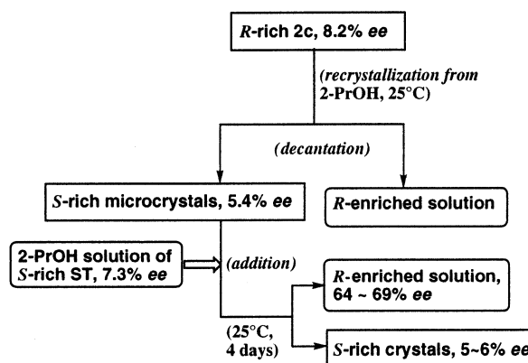
Figure 23. Chiral discrimination by initially formed crystals with a low ee value.
