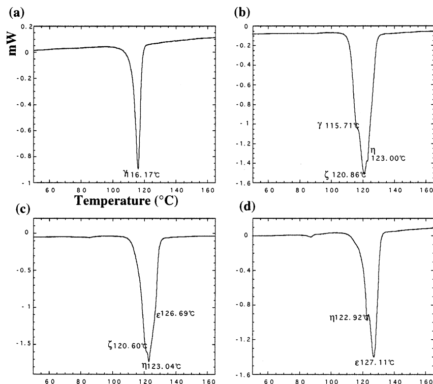
Figure 13. DSC aspects of gradual polymorphic transition of the deposited crystals observed during crystallization of (±)- 1d from EtOH: (a) \gamma -form, (b) a mixture of \gamma , \zeta , and \eta -forms after 8 days, (c) a mixture of \zeta , \eta and \epsilon -forms after 13 days, and (d) a mixture of \eta and \epsilon -forms after 19 days. The endothermic peak at ca. 85 °C corresponds to the desorption of EtOH remaining around the crystals.
