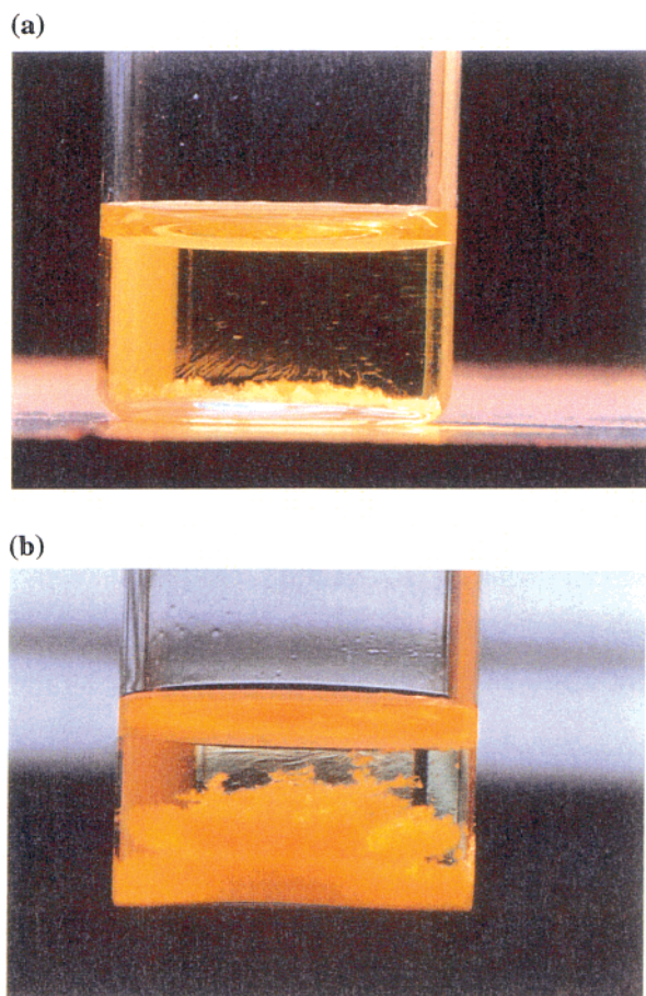
Figure 4. Visual observation of polymorphic transition and redissolution of one enantiomer from the once formed crystals during crystallization from the supersaturated EtOH solution of (±)- 1a (0.1 mol/L); (a) 15 min and (b) 60 min after crystallization began.
