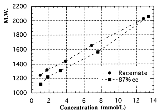
Figure 11. Number-averaged molecular weight measurement of the racemate and nonracemic sample of 2c in \text{CHCl}_3 at 30 °C by vapor pressure osmometry.
