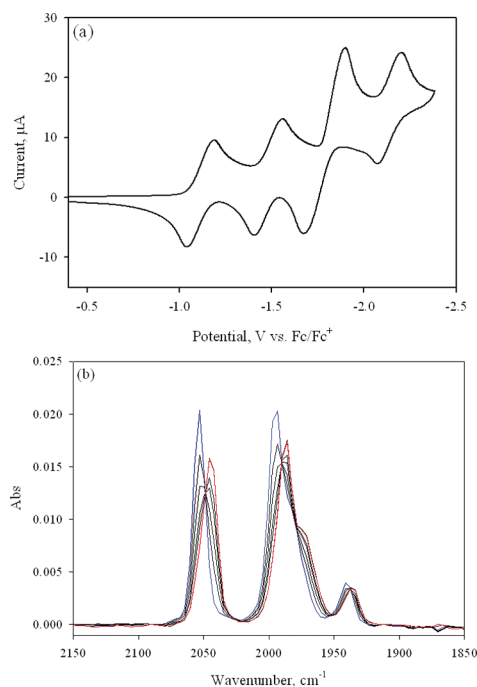
Figure 3. (a) Cyclic voltammogram of 1 (1 mM) in the CH_2Cl_2/o -DCB solution ( \nu = 100 mV/s, 0.1 M n\text{-Bu}_4\text{NPF}_6 ) at 256 K. (b) Spectral changes from 1 (blue line) to [3]^- (red line) monitored by in situ IR spectroscopy in tetrahydrofuran at -50^\circ\text{C} .
