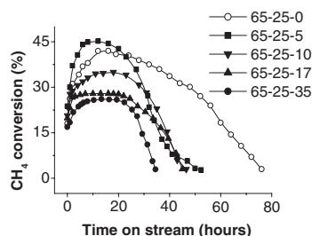
Figure 2. Methane conversion with time on stream over various Ni–Cu–Nb 2 O 5 catalysts at 873 K: (○) GHSV = 24000 mLg -1 h -1 ; (■), (▼), (▲), and (●) GHSV = 48000 mLg -1 h -1 .
