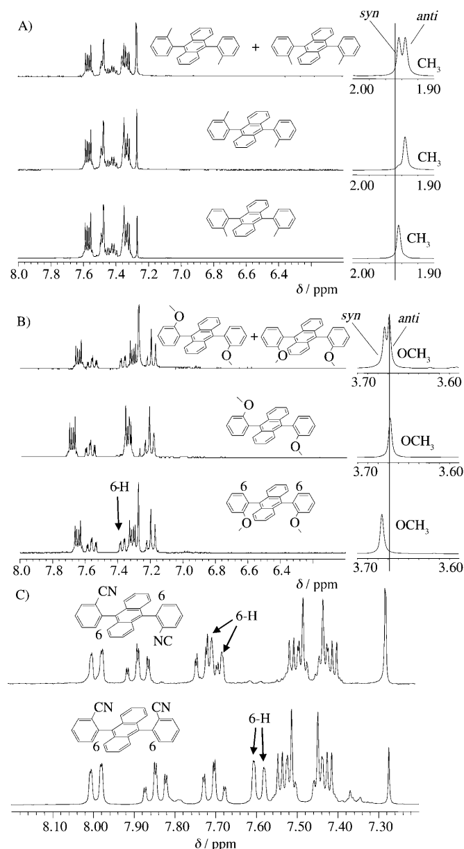
Figure 2. ^1\text{H} NMR spectra of isolated syn and anti isomers of the anthracenes: A) 3a , B) 3d and C) 3f .
