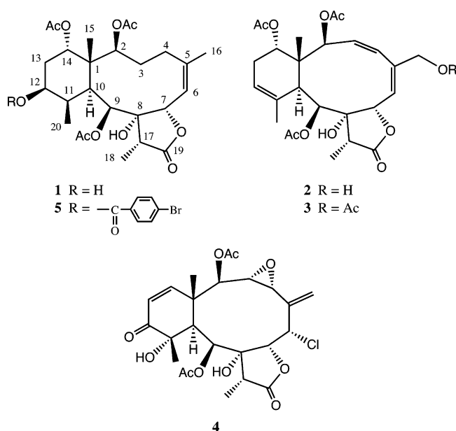
Figure 1. Structures of new diterpenoids.
