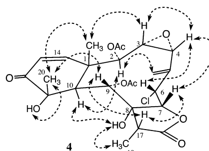
Figure 9. Key NOE correlations (broken arrows) and possible conformation for pachyclavulide D ( 4 ).
