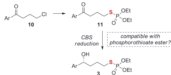
Scheme 2. Proposed Synthesis of Requisite Chiral Alcohol
