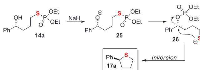
Scheme 7. Proposed Mechanism
