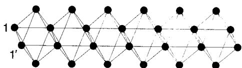
FIG. 2. Chain of trans edge sharing metal octahedra extracted from the structure of \text{Y}_2\text{Cl}_3 . 1 and 1' label the metal atoms in a shared edge.
