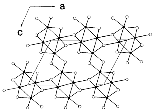
FIG. 1. Structure of \text{Y}_2\text{Cl}_3 projected down [010] of the monoclinic cell. Full circles: Y atoms; open circles: Cl atoms.
