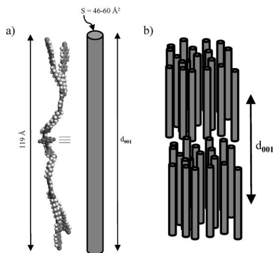
Fig. 2 (a) Simple molecular model for [\text{Ln}(\text{L4})(\text{NO}_3)_3] ( \text{Ln} = \text{Lu}, \text{Tb}, \text{Gd} and \text{Eu} ) in the unit cell. (b) Arrangement of [\text{Ln}(\text{L4})(\text{NO}_3)_3] in the SmA mesophase.
