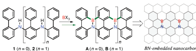
Scheme 1. Tandem Intramolecular Electrophilic Arene Borylation To Synthesize BN-Fused PAHs
