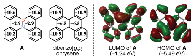
Figure 4. NICS(1) values of A and dibenzo[ g,p ]chrysene, and the Kohn–Sham LUMO and HOMO of A at the B3LYP/6-31G* level.
