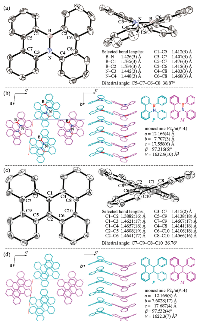
Figure 1. ORTEP drawing and packing structure of A (a,b) and dibenzo[ g,p ]chrysene (c,d). Thermal ellipsoids are shown at 50% probability; hydrogen atoms are omitted for clarity. ( P )-enantiomer, blue; ( M )-enantiomer, pink.
