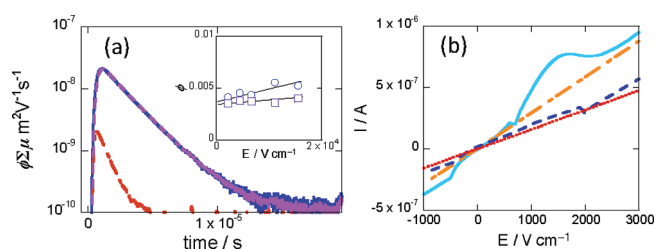
Figure 2. (a) Conductivity transients monitored for the polycrystalline phase of A in Ar (blue) and SF 6 (violet) environments. Identical traces were observed for both atmospheres. The kinetic trace for transient conductivity was also observed for dibenzo[ g,p ]chrysene (red). Excitation was carried out at 355 nm using 13 \text{ mJ cm}^{-2} pulses for all transients. Dependence of \phi on the applied electric field strength between interdigitated Au electrodes with a 5\text{-}\mu\text{m} gap. The values of \phi were determined by photocurrent integration under illumination of a thin film of A (120 nm thick) and dibenzo[ g,p ]chrysene (80 nm thick) at 355 nm, 22 \text{ mJ cm}^{-2} . The photocurrent under 355-nm illumination was also traced using identical samples; the I – V traces are illustrated in (b). Blue dashed and red dotted lines are the traces of A (dark and illuminated, respectively), and turquoise solid and orange dot-dashed lines are the traces of dibenzo[ g,p ]chrysene (dark and illuminated, respectively).
