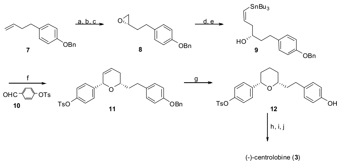
Scheme 3. Reagents and conditions: (a) AD-mix- \alpha , t -BuOH–H 2 O, 0 °C, 80%, 90% ee; (b) TsCl, pyridine, 0 °C, 88%; (c) NaOH, Et 2 O–H 2 O, 93%; (d) lithium acetylide–EDA, DMSO, 0 °C, 83%, 87% ee; (e) Bu 2 Sn(OTf)H then n -BuLi, 72%; (f) 10 , TMSOTf (2.0 equiv), Et 2 O, –78 °C, 87%; (g) Pd/C, H 2 , EtOAc, 78%; (h) TBSCl, imidazole, 95%; (i) Mg (10 equiv), MeOH, 25 °C, 50%; (j) NaH, MeI, THF then Bu 4 NF, THF, 0 °C, 73% (over two steps).
