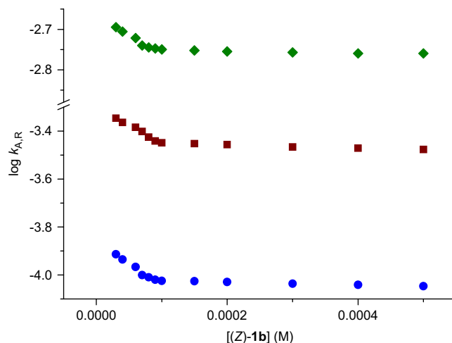
Figure 2. Plot of \log k_{A,R} for the rearrangement of (Z)- 1b into 2b in D/W versus concentration of (Z)- 1b at \text{pS}^+ 10.80 (●), 11.38 (■), and 12.10 (◆).
