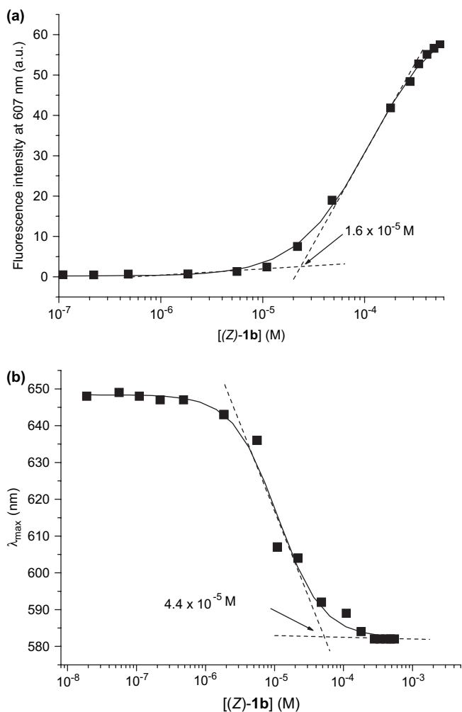
Figure 6. (a) Plot of the fluorescence intensity (arbitrary units) versus the concentration of (Z)- 1b . (b) Plot of the \lambda_{\max} (nm) versus the concentration of (Z)- 1b .
