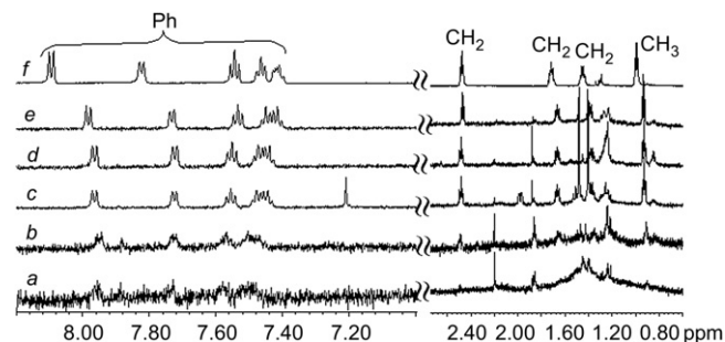
Figure 5. ^1\text{H} NMR spectra of a 1.2\times 10^{-4} M solution of 2a recorded at T 298 K in solution of \text{D}_2\text{O}/\text{CD}_3\text{OD} (v/v): (a) 6:1, (b) 4:1, (c) 1.5:1, (d) 1.2:1, (e) 1:1.75, (f) 0:1.
