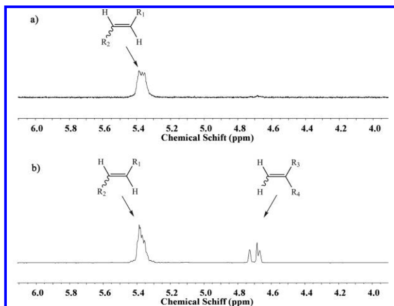
Figure 5. ^1\text{H} NMR spectrum of the end groups for oligo(1-hexene)s produced by (a) the zirconium catalyst 9 /MAO (Table 3, run 11) and (b) the zirconium catalyst 7 /MAO (Table 3, run 7).
