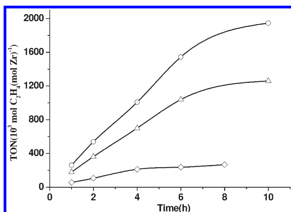
Figure 4. Lifetime plot of ethylene polymerization for complexes 7 (M), 8 (8) and 9 (—) at 20 °C. Reaction conditions: zirconium complex 0.2 \mu mol, MAO 0.2 mmol, ethylene 5 bar, toluene 100 mL.
