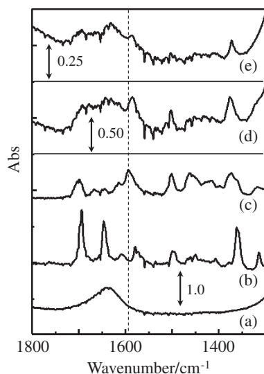
Figure 4. IR spectra of (a) \text{Fe}^{3+} -Mica, (b) AIP 2 , (c) 2\text{-FeCl}_3 complex, (d) precatalyst 2 ( 560\ \mu\text{mol-2/g-Fe}^{3+} -Mica), and (e) precatalyst 2 ( 200\ \mu\text{mol-2/g-Fe}^{3+} -Mica).
