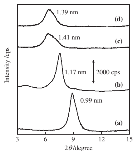
Figure 3. XRD profiles of (a) Fe 3+ -Mica (dried at 200 °C under reduced pressure), (b) Fe 3+ -Mica (treated only with CH 3 CN), (c) precatalyst 1 , and (d) precatalyst 2 . The profiles of samples (b)–(d) were measured after drying at 110 °C under reduced pressure.
