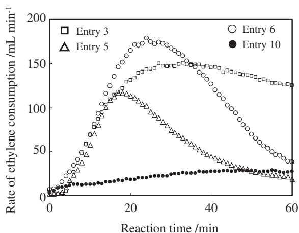
Figure 2. Profiles of ethylene consumption using heterogeneous (precatalyst 2 /R' 3 Al) and homogeneous ( 2 -FeCl 3 /MAO) catalysts.
