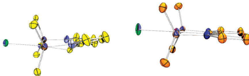
Figure 4. POV-Ray 12 renditions of the Ortep drawings 13 (50% probability ellipsoids) of 2 (left) and 9-PF 6 (right) viewed along the P–Pd–P axis. Omitted for clarity: H atoms, methyls of the 1 Pr groups, PF 6 − group.
