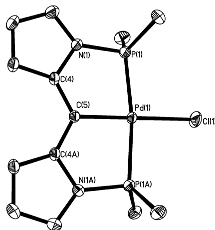
Figure 3. ORTEP drawing (50% thermal ellipsoids) of 9-PF 6 showing selected atom labeling. Hydrogen atoms, methyl groups, and the counteranion (PF 6 ) are omitted for clarity. Selected bond distances (Å) and angles (deg): Pd1–P1A 2.2730(7); Pd1–P1 2.2730(7); Pd1–Cl1 2.3337(11); Pd1–C5 1.999(4); P1A–Pd1–P1 171.30(4); P1A–Pd1–Cl1 94.35(2); P1–Pd1–Cl1 94.35(2); P1A–Pd1–C5 85.65(2); P1–Pd1–C5 85.65(2); Cl1–Pd1–C5 179.99(4).
