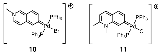
Chart 3. “Remote” NHC Complexes of Pd
