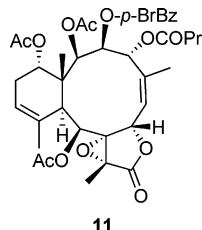
Figure 2. Structure of p -bromobenzoate 11 .
