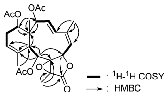
Figure 7. Selective ^1\text{H} - ^1\text{H} COSY and HMBC correlations of 9 .
