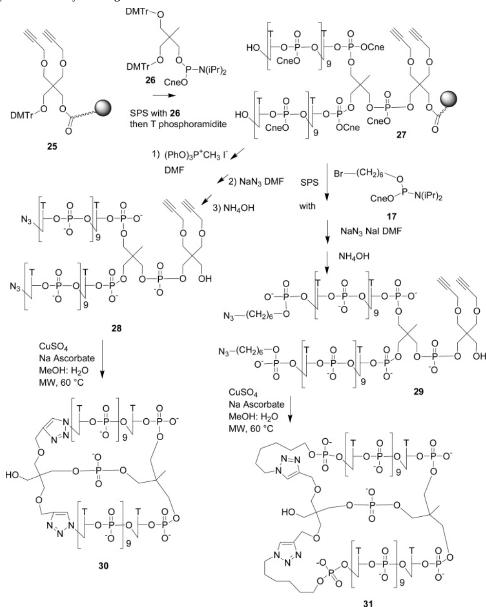
SCHEME 9. Synthesis of Bicyclic Oligonucleotides 30 and 31
