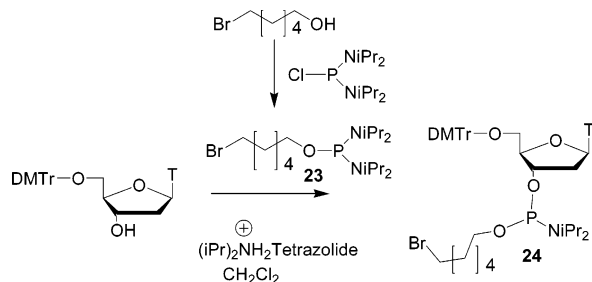
SCHEME 8. Synthesis of Bromohexyl Phosphoramidite of Thymidine
