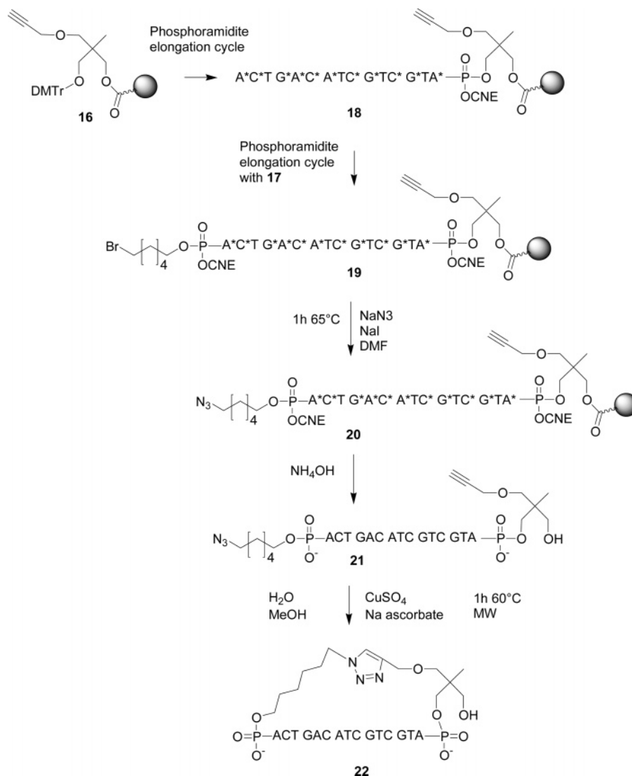
SCHEME 7. Universal Method for Cyclic Oligonucleotide Synthesis by MW-CuAAC Reaction a
