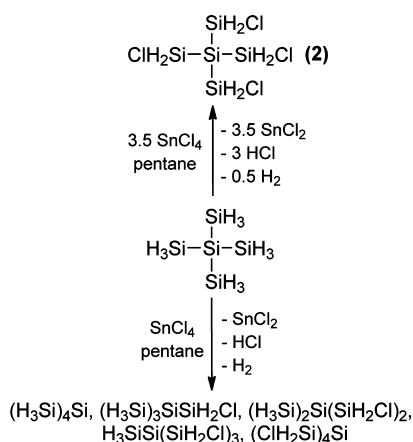
Scheme 2. Chlorination of Neopentasilane (\text{H}_3\text{Si})_4\text{Si} with \text{SnCl}_4
