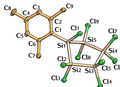
Figure 2. Molecular structure of 3 in the crystal (50% thermal probability ellipsoids). Selected bond lengths (Å), angles (deg), and torsion angles (deg) with estimated standard deviations: Si1–Si2 2.365(1), Si1–Si5 2.353(1), Si2–Si3 2.367(1), Si3–Si4 2.360(1), Si4–Si5 2.352(1), Si1–Cl1 1.867(2), Si1–Cl1 2.123(1), \text{Si}_{\text{in}}-\text{Cl} (mean) 2.050; Si5–Si1–Si2 98.7(1), Si1–Si2–Si3 103.2(1), Si4–Si3–Si2 106.4(1), Si5–Si4–Si3 103.4(1), Si4–Si5–Si1 103.8(1); Si1–Si2–Si3–Si4 24.7(1), Si2–Si3–Si4–Si5 5.4(1), Si3–Si4–Si5–Si6 33.8(1), Si4–Si5–Si1–Si2 48.7(1), Si5–Si1–Si2–Si3 44.3(1).
