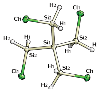
Figure 1. Molecular structure of 2 in the crystal (50% thermal probability ellipsoids). Selected bond lengths (Å) and angles (deg) with estimated standard deviations: Si1–Si2 2.346(1) , Si2–Cl1 2.074(1) ; Si2–Si1–Si2 111.4(1) , 111.4(1) , 111.4(1) , 105.7(1) , 105.7(1) , Cl1–Si2–Si1 108.8(1) .
