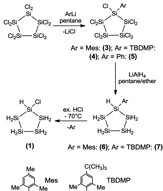
Scheme 3. Selective Monofunctionalization of Cyclopentasilane \text{Si}_5\text{H}_{10}
