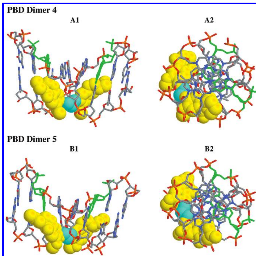
Figure 3. Energy-minimized models for the minor groove cross-linked adducts formed with d(CGCA G ATCTGCG) 2 and either 4 (A1, A2) or the more extended dimer 5 (B1, B2). Only the central eight base pairs are shown for each structure with all hydrogen atoms removed for clarity. The bound molecules are highlighted in space fill; color scheme: PBD subunits (yellow), inert ligand C8–C8' diether linkage (cyan), and alkylated guanine bases (green). Panels A2 and B2 represent views looking down the long dyad or z -axis of the DNA duplex, showing the effective burial of the dimer molecules within the minor groove conduit. The only exposed molecular fragments are the 7-methoxy substituents in each PBD A-ring.
