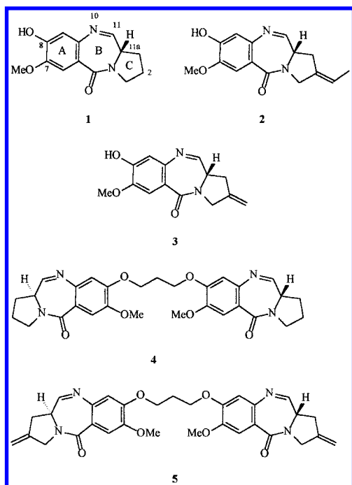
Figure 1. Structures of the PBD monomers DC-81 ( 1 ), tomaymycin ( 2 ), and C2-methylene DC-81 ( 3 ), and the PBD dimers 4 and 5 .
