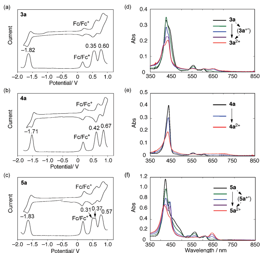
Figure 4. (a)–(c) Cyclic voltammograms (upper) and differential pulse voltammograms (lower) in the range of -2.0 to 1.0 V for (a) 3a , (b) 4a , and (c) 5a . Measured in \text{CH}_2\text{Cl}_2 with 0.1 M \text{Bu}_4\text{NPF}_6 as a supporting electrolyte; \text{Ag}/\text{Ag}^+ [\text{AgNO}_3 (\text{MeCN})] as a reference electrode; Scan rate 20 mV \text{s}^{-1} . Redox potentials (in V) relative to that of \text{Fc}/\text{Fc}^+ are shown above DPV voltammograms. (d)–(f) Spectroscopic changes observed in the electrochemical oxidation processes from (d) 3a , (e) 4a , and (f) 5a to their dication species in \text{CH}_2\text{Cl}_2 containing 0.1 M of \text{Bu}_4\text{NPF}_6 .
