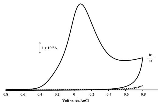
Figure 4. Cyclic voltammogram of 0.1 mM 3 at a GC electrode in \text{CH}_3\text{CN}/0.1\text{ M } [\text{Bu}_4\text{N}]\text{PF}_6 at 100 mV/s versus \text{Ag}/\text{AgCl} . Top: Reduction at the first cycle. Bottom: Reduction at the second cycle.
