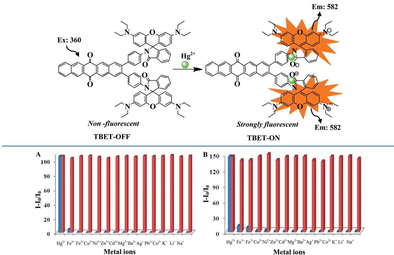
Figure 3. (A) Fluorescence response of receptor 5 ( 10\ \mu\text{M} ) upon the addition of various cations (200 equiv) in THF/ \text{H}_2\text{O} (9.5:0.5, v/v) buffered with HEPES, pH = 7; \lambda_{\text{ex}} = 360 nm. (B) Fluorescence response of receptor 8 ( 10\ \mu\text{M} ) upon the addition of various cations (200 equiv) in THF/ \text{H}_2\text{O} (9.5:0.5, v/v) buffered with HEPES, pH = 7; \lambda_{\text{ex}} = 360 nm. Bars represent the emission intensity ratio ( I - I_0/I_0 ). I_0 is the fluorescence intensity of each free host, and I is the fluorescence intensity after the addition of metal ions. The blue bars represent the addition of various metal ions, while the red bars represent the change in the emission that occurs upon the subsequent addition of \text{Hg}^{2+} (200 equiv) to the above solution.
