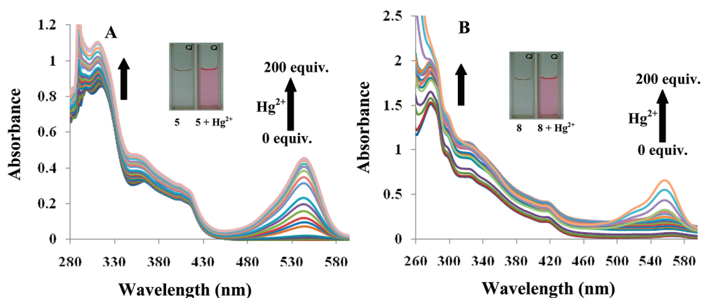
Figure 1. (A) UV-vis spectra of 5 (10 \mu M) in the presence of \text{Hg}^{2+} ions (0–200 equiv) in THF/ \text{H}_2\text{O} (9.5:0.5, v/v) buffered with HEPES, pH = 7. Inset: Change in the color of the receptor before and after the addition of \text{Hg}^{2+} ions. (B) UV-vis spectra of 8 (10 \mu M) in the presence of \text{Hg}^{2+} ions (0–200 equiv) in THF/ \text{H}_2\text{O} (9.5:0.5, v/v) buffered with HEPES, pH = 7. Inset: Change in the color of the receptor before and after the addition of \text{Hg}^{2+} ions.
