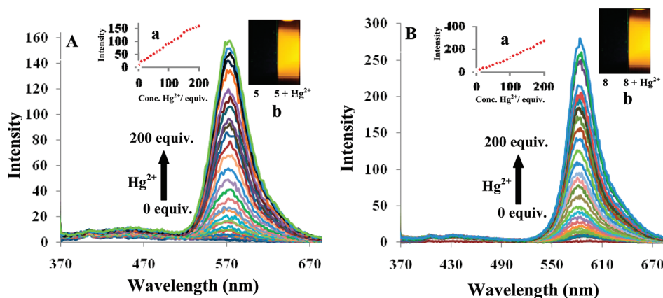
Figure 2. (A) Fluorescence response of receptor 5 (10 \mu M) upon the addition of \text{Hg}^{2+} ions (0–200 equiv) in THF/ \text{H}_2\text{O} (9.5:0.5, v/v) buffered with HEPES, pH = 7; \lambda_{\text{ex}} = 360 nm. Inset: (a) Change in the fluorescence intensity of receptor 5 as a function of the \text{Hg}^{2+} ion concentration. (b) Fluorescence before and after the addition of \text{Hg}^{2+} ions. (B) Fluorescence response of receptor 8 (10 \mu M) upon the addition of \text{Hg}^{2+} ions (0–200 equiv) in THF/ \text{H}_2\text{O} (9.5:0.5, v/v) buffered with HEPES, pH = 7; \lambda_{\text{ex}} = 360 nm. Inset: (a) Change in the fluorescence intensity of receptor 8 as a function of the \text{Hg}^{2+} ion concentration. (b) Fluorescence before and after the addition of \text{Hg}^{2+} ions.
