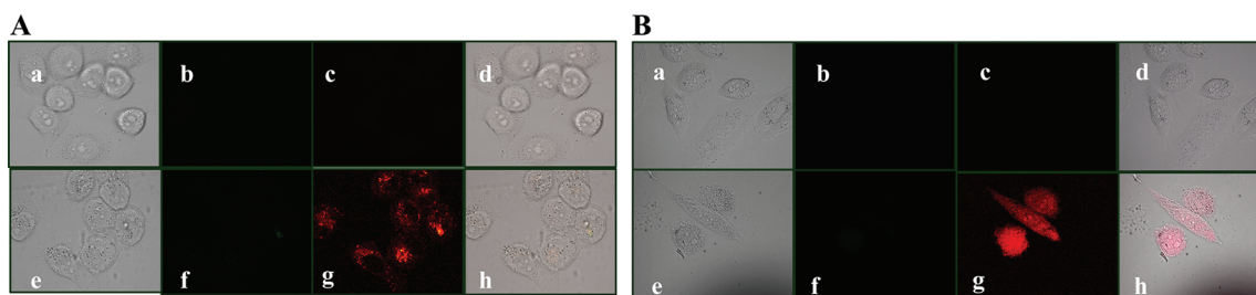
Figure 4. Fluorescence and bright-field images of PC3 cell lines: (a) bright-field image of cells treated with probe 8 ( 1.0\ \mu\text{M} ) only for 20 min at 37\ ^\circ\text{C} ; (b and c) fluorescence images of part a in green and red channels, respectively. (d) Overlay image of parts a–c; (e) bright-field image of cells upon treatment with probe 8 ( 1.0\ \mu\text{M} ) and then with \text{Hg}(\text{ClO}_4)_2 ( 30.0\ \mu\text{M} ) for 20 min; (f and g) fluorescence images of part e in green and red channels, respectively; (h) overlay image of parts e–g. (A) \lambda_{\text{ex}} = 488\ \text{nm} . (B) \lambda_{\text{ex}} = 405\ \text{nm} .
