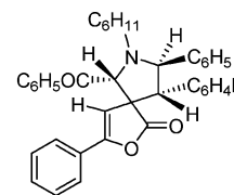
Spiro[butenolide]pyrrolidines (II)
