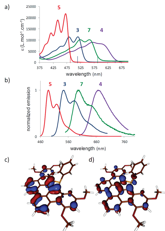
Figure 2. (a) UV-vis absorption and TD-DFT-simulated spectra (vertical lines). (b) Normalized emission spectra of 3 (blue), 4 (purple), 5 (red), and 7 (green) in \text{CH}_2\text{Cl}_2 ( 10^{-5} \text{ M} ). (c, d) Kohn-Sham MOs of 5 : (c) HOMO; (d) LUMO.
