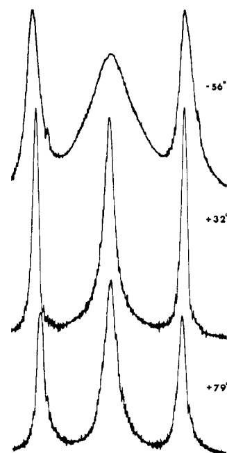
Figure 3. Proton nmr spectra of trans -Fe(CO) 3 [P(N(CH 3 ) 2 ) 3 ] 2 in toluene- d 8 at -56^\circ , +32^\circ , and +79^\circ .
