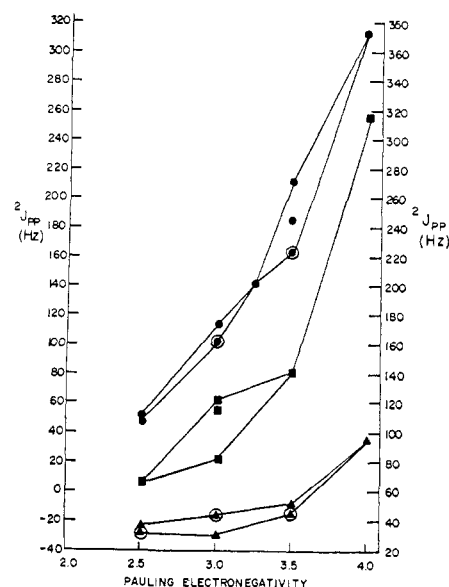
Figure 6. A plot showing the progression of {}^2J_{PP} for trans\text{-}M(\text{CO})_4\text{L}_2 (where M = \text{Cr} ( \blacktriangle ), \text{Mo} ( \bullet ), or \text{W} ( \blacksquare )) as a function of the electronegativity of the ligand. The left ordinate applies to the Cr and Mo complexes and the right to the tungsten systems. See text for the ligands employed and the method of calculating their electronegativity.
