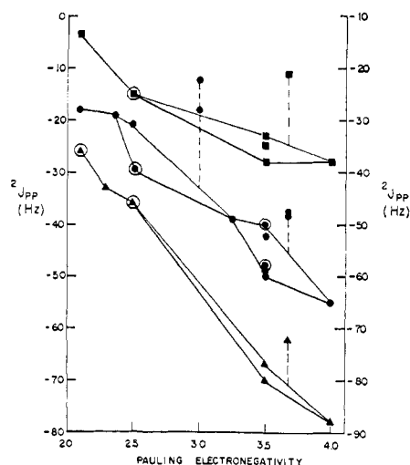
Figure 5. A plot showing the progression of {}^2J_{PP} for cis\text{-}M(\text{CO})_4\text{L}_2 (where M = \text{Cr} ( \blacktriangle ), \text{Mo} ( \bullet ), or \text{W} ( \blacksquare )) as a function of the electronegativity of the ligand. The left ordinate applied to the Cr and Mo complexes and the right to the tungsten systems. See text for the ligands employed and the method of calculating their electronegativity.
