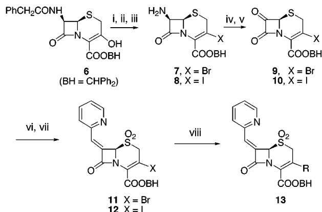
Scheme 3. New Synthetic Route Employing 3-Halo-7-alkylidenecephem Sulfones a
