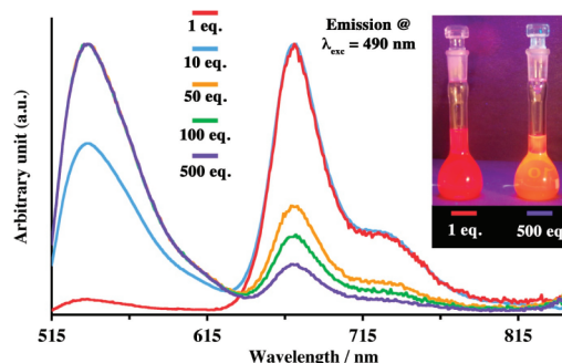
Figure 2. Fluorescence changes at rt, c = 1 \times 10^{-6} M, by successive addition of TBAP in THF. \lambda_{\text{exc}} = 490 nm.
