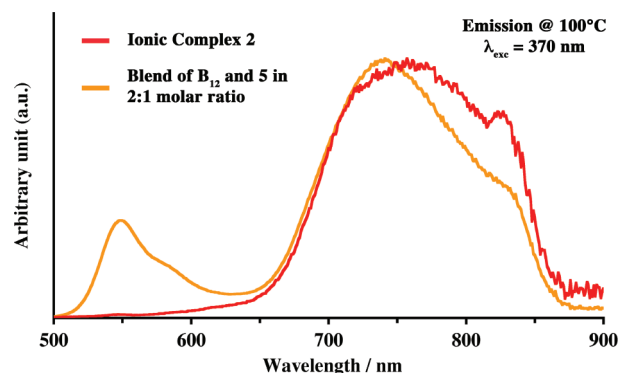
Figure 3. Fluorescence spectrum ( \lambda_{\text{exc}} = 370 nm) of complex 2 in the columnar mesophase at 100 °C (red trace). Fluorescence spectrum ( \lambda_{\text{exc}} = 370 nm) of complex B12 mixed with dye 5 in a 2 to 1 mol stoichiometry in the solid state at 100 °C (orange trace).
