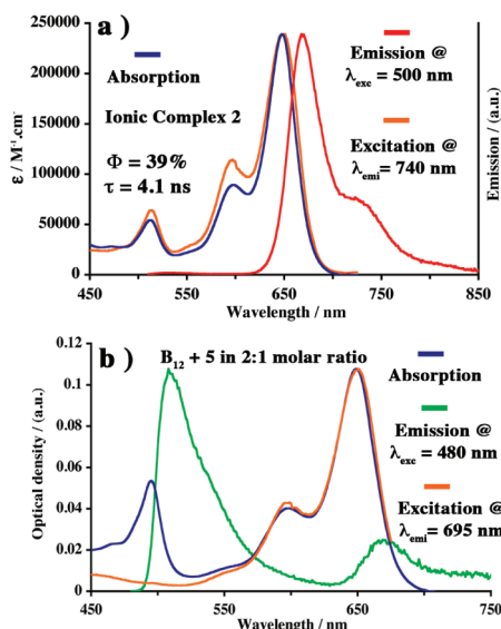
Figure 1. Absorption, fluorescence, and excitation spectra in THF, at rt, c = 1 \times 10^{-6} M: (a) complex 2 ( \lambda_{\text{exc}} = 500 nm, \lambda_{\text{em}} = 740 nm), (b) 2/1 mixture of B 12 and dye 5 ( \lambda_{\text{exc}} = 480 nm, \lambda_{\text{em}} = 695 nm).
