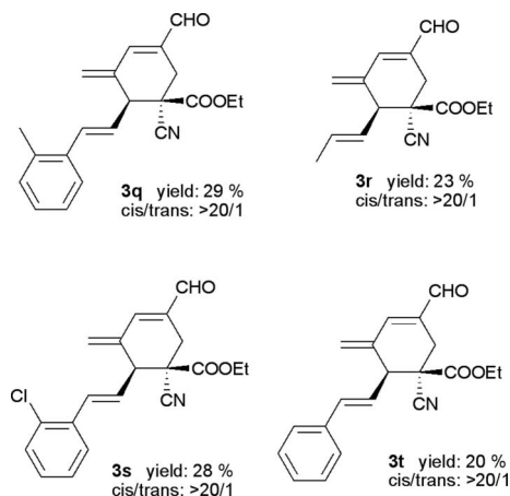
Fig. 3 Triple domino reaction of conjugated dienes 1 with acrolein 2 .
