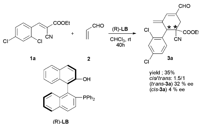
Scheme 4 Asymmetric annulation.
