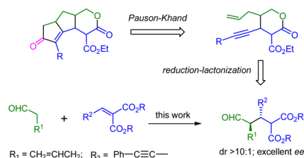
Scheme 2. Retrosynthetic Analysis
