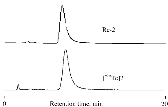
Figure 3. Reversed-phase HPLC chromatogram of Re-2 and [ ^{99m}\text{Tc} ]2. Conditions: PRP-1 column, 250 \times 4.1 mm; \text{CH}_3\text{CN}/3,3 -dimethylglutarate buffer, 5 mM, pH 7, volume ratio 9 : 1; flow rate 1 ml/min. Re-2 was monitored at 254 nm
