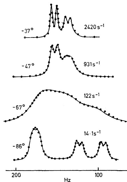
Experimental (●) and 'best fit' computed (solid line) band-shapes for the isopropyl methyl signals of NN -di-isopropyl- P -phenylphosphonamidothioic chloride (2) at various temperatures in \text{CHCl}_2\text{F} solution. The calculated site exchange rates are also shown
