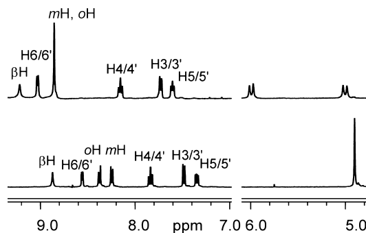
Figure 4. Comparison of ^1\text{H} NMR spectra of \text{T}(N(\text{SO}_2\text{C}_6\text{H}_4)\text{dpa})\text{P} (bottom) and [[\text{Re}(\text{CO})_3]_4\text{T}(N(\text{SO}_2\text{C}_6\text{H}_4)\text{dpa})\text{P}](\text{BF}_4)_4 ( 6 ) (top) in \text{DMSO}-d_6 at 25^\circ\text{C} .
