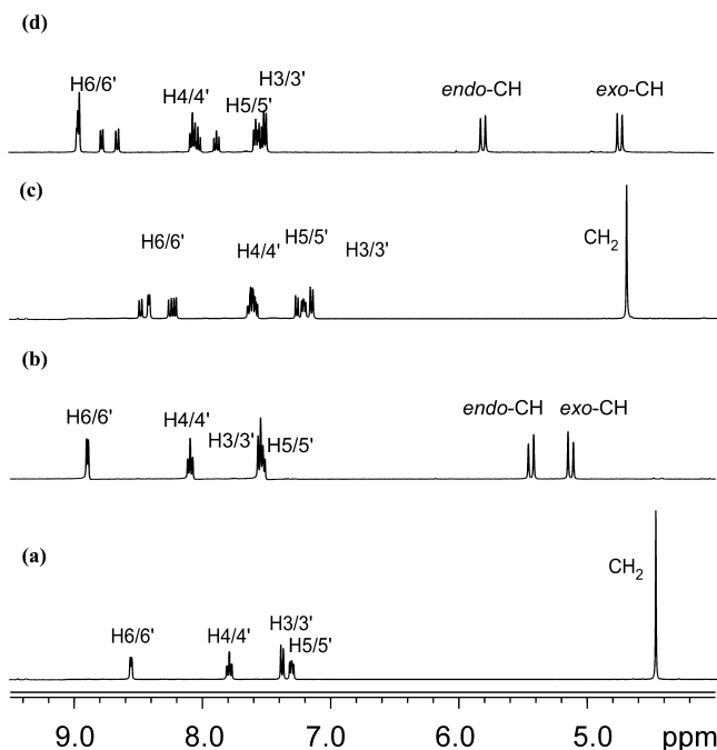
Figure 3. Comparison of the 1 H NMR spectra of ligands N(SO 2 Me)dpa (a), N(SO 2 Me 2 Nnap)dpa (c) and the corresponding Re complexes ([Re(CO) 3 (N(SO 2 Me)dpa)]PF 6 ( 1 ) (b), [Re(CO) 3 (N(SO 2 Me 2 Nnap)dpa)]BF 4 ( 5 ) (d)) in DMSO- d 6 at 25 °C.
