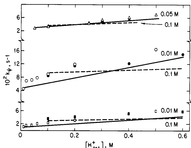
Figure 3. Hydrolysis of the acetals 2a,b with added HCl: \Delta , 2b and 0.05 M 1b ; \triangle , 2a and 0.1 M 1b ; \square , 2b and 0.01 M 1c ; \blacksquare , 2b and 0.1 M 1c . The solid lines are predicted for the lower and the broken lines for the higher surfactant concentrations.
