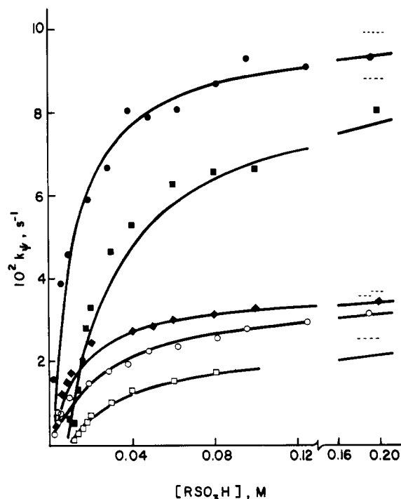
Figure 2. Hydrolyses of the acetals 2a,b . Open points denote 2a , closed 2b . ♦, 1a ; ■, 1b ; ●, 1c . The solid lines are predicted, and the broken lines are predicted k_p at total substrate incorporation.
