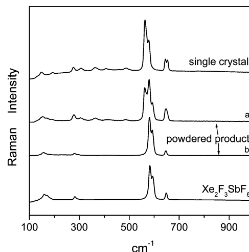
Figure 7. Raman spectrum of [\text{Cu}(\text{XeF}_2)_4](\text{SbF}_6)_2 (recorded on a single crystal), Raman spectra of the powdered product of reaction between \text{Cu}(\text{SbF}_6)_2 and 4\text{XeF}_2 recorded on different spots of the same sample [(a) mixture of [\text{Cu}(\text{XeF}_2)_2](\text{SbF}_6)_2 and \text{Xe}_2\text{F}_3\text{SbF}_6 , (b) \text{Xe}_2\text{F}_3\text{SbF}_6 only], and the Raman spectrum of pure \text{Xe}_2\text{F}_3\text{SbF}_6 .
