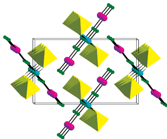
Figure 4. Packing of the -\text{[Cu}(\text{XeF}_2)_2]\text{-(SbF}_6)_2\text{-[Cu}(\text{XeF}_2)_2]\text{-} chains in the crystal structure of [\text{Cu}(\text{XeF}_2)_2](\text{SbF}_6)_2 .
