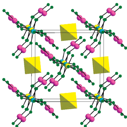
Figure 2. Packing of -\text{[Cu}(\text{XeF}_2)_4]\text{-(SbF}_6)_2\text{-[Cu}(\text{XeF}_2)_4]\text{-} chains and free [\text{SbF}_6] units in the crystal structure of [\text{Cu}(\text{XeF}_2)_4](\text{SbF}_6)_2 .
