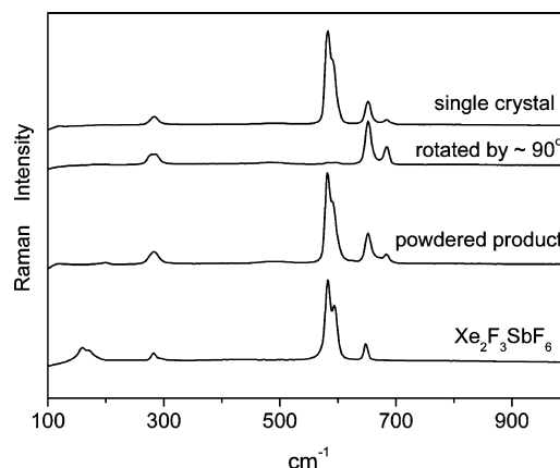
Figure 6. Raman spectra of [\text{Cu}(\text{XeF}_2)_2](\text{SbF}_6)_2 (recorded on a single crystal at different orientations), Raman spectrum of the powdered product of reaction between \text{Cu}(\text{SbF}_6)_2 and 2\text{XeF}_2 , and Raman spectrum of \text{Xe}_2\text{F}_3\text{SbF}_6 .
