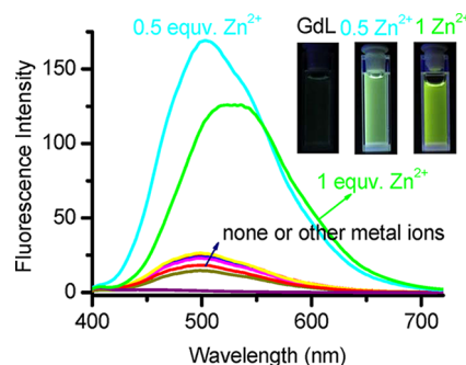
Figure 4. Fluorescence spectra of GdL (20 \mu\text{M} ) in the presence of 0.5 or 1 equiv of \text{Zn}^{2+} , and 1 equiv of \text{K}^+ , \text{Na}^+ , \text{Ca}^{2+} , \text{Mg}^{2+} , \text{Fe}^{2+} , \text{Fe}^{3+} , and \text{Cu}^{2+} in 100 mM HEPES buffer solutions at 25 °C, pH = 7.2 ( \lambda_{\text{ex}} = 360 nm). Inset luminescence photographs were taken from 50 \mu\text{M} GdL solutions in the absence and presence of 0.5 or 1 equiv of \text{Zn}^{2+} under UV light irradiation at 365 nm.
