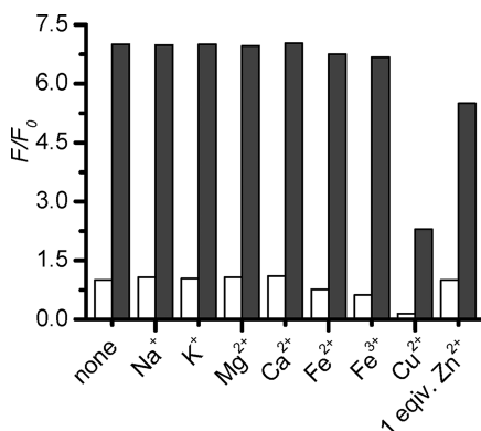
Figure 5. Fluorescence ( \lambda_{\text{ex}} = 360 nm) intensity of GdL ( 20 \mu\text{M} ) in the presence of 0.5 equiv of biological metal ions (blank bars), or 0.5 equiv of \text{Zn}^{2+} together with 0.5 equiv of an interfering metal ion (shadow bars). The last two bars represent the fluorescence intensity of GdL ( 20 \mu\text{M} ) in the absence (blank bar) and presence (shadow bar) of 1 equiv of \text{Zn}^{2+} .
