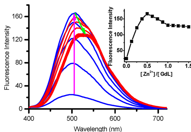
Figure 7. Emission spectral changes of GdL ( 20 \mu\text{M} ) upon addition of \text{Zn}^{2+} ( [\text{Zn}^{2+}] = 0, 2.5, 5, 7.5, 10, 12.5, 15, 17.5, 20, 22.5, 25, 27.5, and 30 \mu\text{M} ) in 100 mM HEPES buffer solutions at 25^\circ\text{C} , pH = 7.2 ( \lambda_{\text{ex}} = 360 nm).
