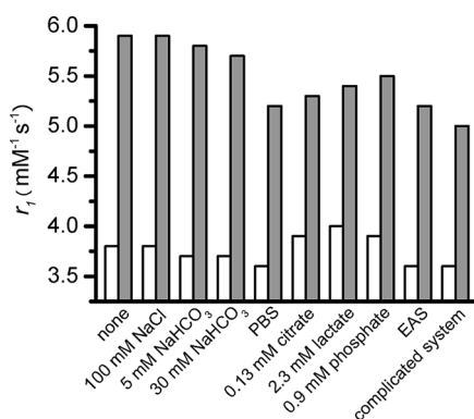
Figure 3. Relaxivity response of GdL to 0.5 equiv of \text{Zn}^{2+} at 23 MHz in the presence of biologically relevant anions. Blank bars represent the relaxivity of GdL in the presence of corresponding anions. Shadow bars represent the relaxivity upon addition of 0.5 equiv of \text{Zn}^{2+} to GdL in presence of corresponding anions. All measurements were performed in 100 mM HEPES buffer, pH = 7.2 except for PBS, EAS, and the complicated system. The relaxivity measurement with PBS was acquired under similar conditions using PBS, pH = 7.4. EAS contains 30 mM \text{NaHCO}_3 , 100 mM \text{NaCl} , 0.9 mM \text{KH}_2\text{PO}_4 , 2.3 mM sodium lactate, and 0.13 mM sodium citrate, pH = 7.0. A complicated solution system contains all the anions in EAS as well as 5 mM \text{KCl} , 2 mM \text{CaCl}_2 , 0.7 mM \text{MgCl}_2 , 0.5 mM \text{FeCl}_2 , 0.5 mM \text{FeCl}_3 , and 0.1 mM \text{CuCl}_2 , pH = 7.0.
