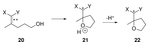
Scheme 5. Distonic Radical Cation 21 Not at a Local Energy Minima a
