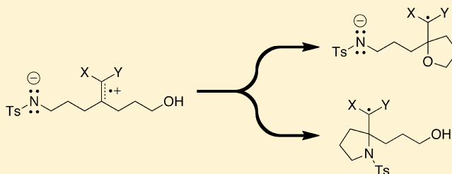
Scheme 1. General Design of a Competition Study a
