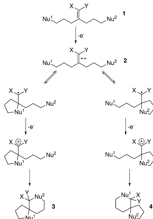
Scheme 1. General Design of a Competition Study a
