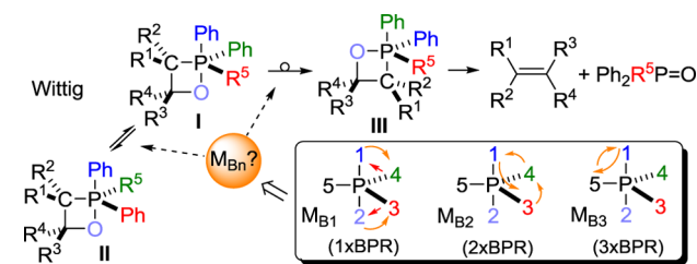
Scheme 1. Possible Stereomutation Mechanisms in the Wittig Reaction
