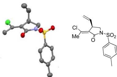
Figure 1. Structure determination for compound (+)- 2a by X-ray crystallographic analysis.
