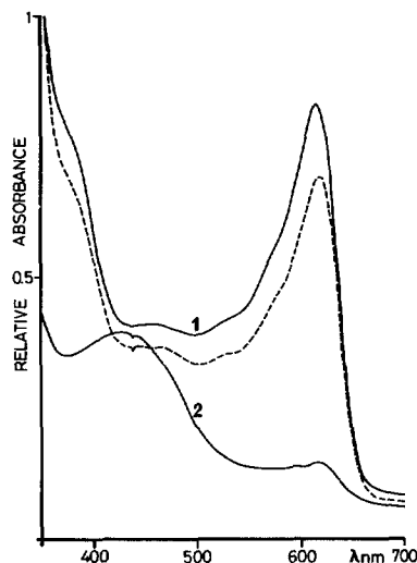
Fig. 1. UV-Vis absorption spectra of an \text{Fc}^{++} solution in acetonitrile propanol-1 (1.25:1) mixture: curve 1, before photolysis; curve 2, after photolysis; -----, blank solution.
