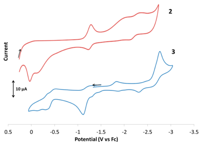
Figure 2. CVs of complexes 2 and 3 (2 mM analyte in 0.4 M [\text{nBu}_4\text{N}][\text{PF}_6] in THF, scan rate = 100 mV/s).
