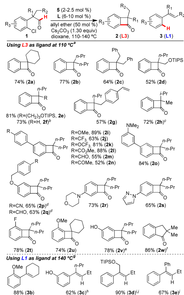
Scheme 3. Reaction Scope
